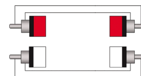
Unbalanced connection
