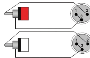
Balanced connection
