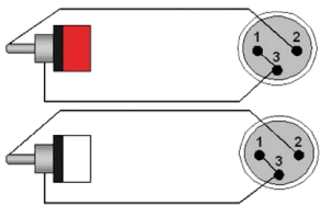
Balanced connection
